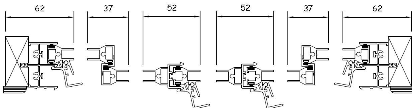
Section B-B.
