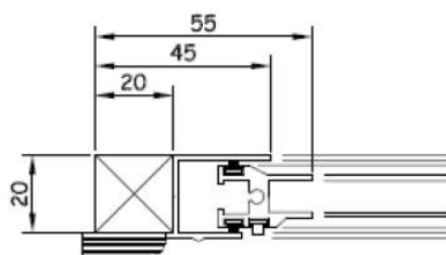
Lift Out Jamb detail.
