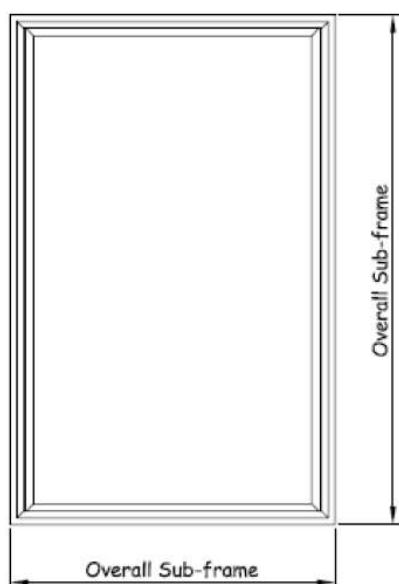
Typical elevation of a Slim Line Lift Out frame.
