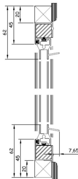
Section through the Lift Out frame.
