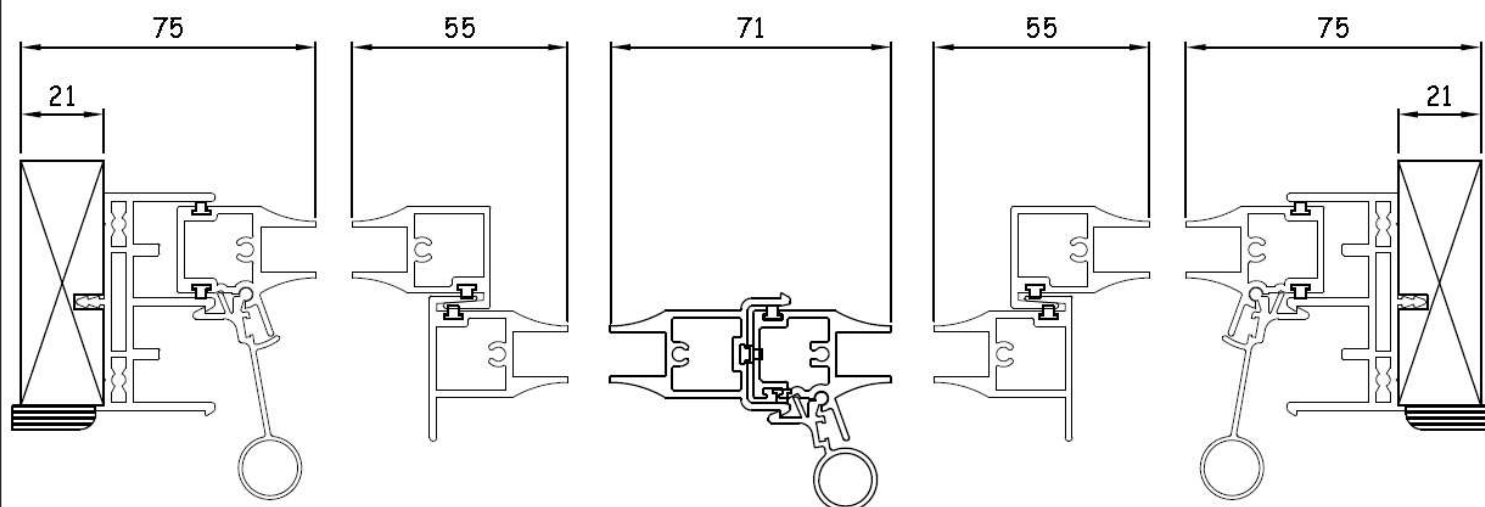
Section B-B detail.
