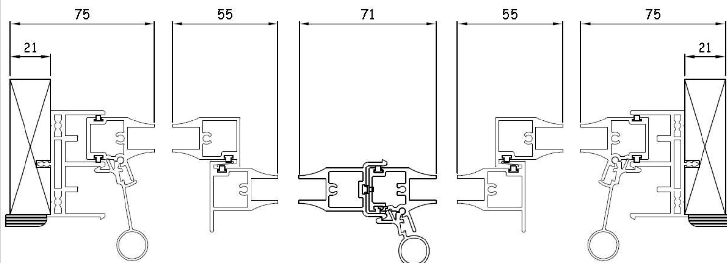
Section B-B detail.
