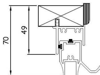
Section A-A detail.
