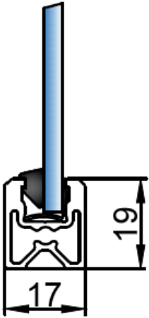
Standard Frame 4mm to 6.6mm glass sizes
