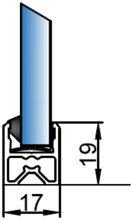
Ultra-Frame 8mm to 10.8mm glass sizes
